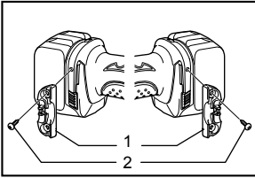
1. Chuck key holder 2. Screw
