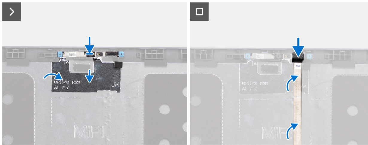
Figur 67. Installera kameran
