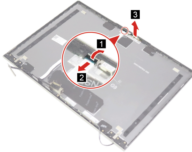
Figure 61. Disconnect the EDP cable and remove the camera board
