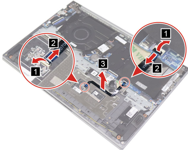
Figure 10. Disconnect and remove the touchpad board cable
