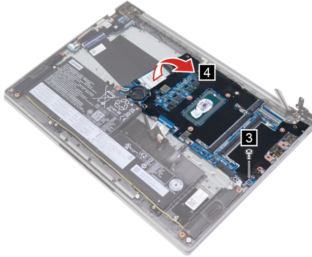
Figure 32. Remove one screw and remove the system board
