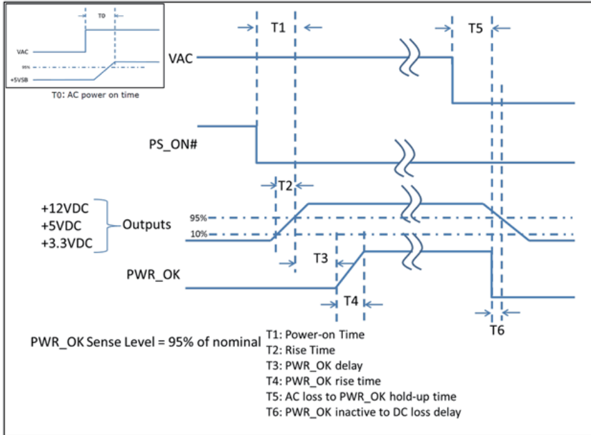
Figure 1 Time Diagram
