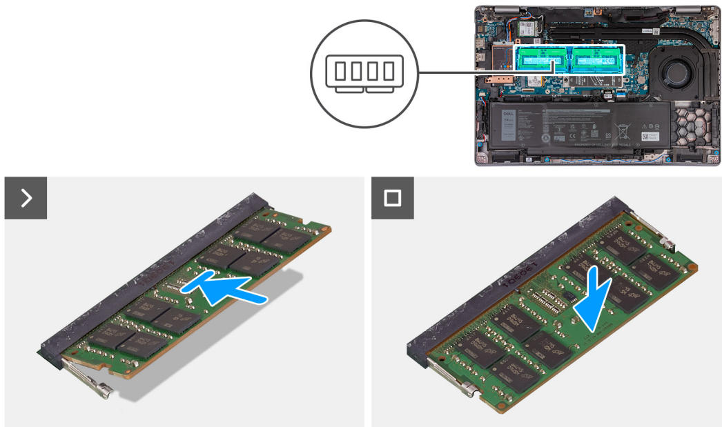
Figur 26. Installera minnesmodulen
