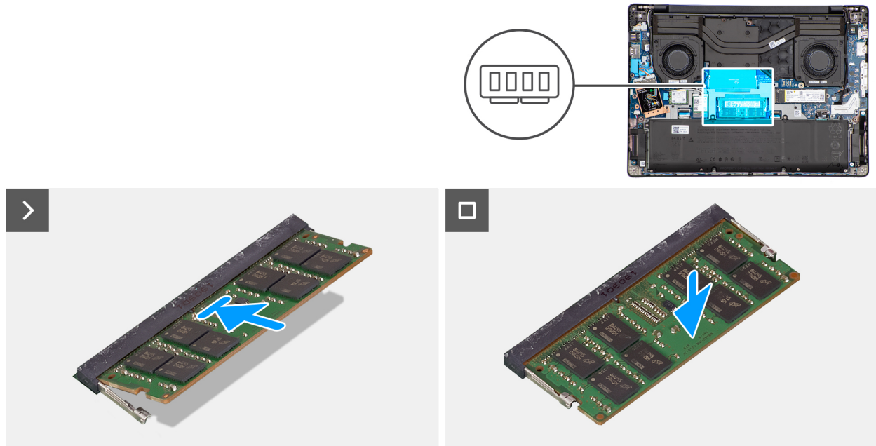
Figur 22. Installera minnesmodulen
