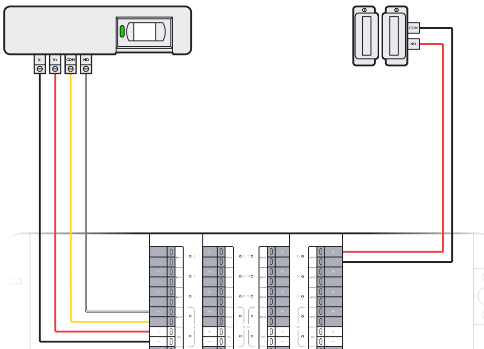
Third-Party Motion Sensor
